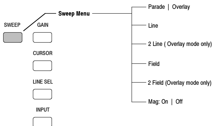
Figure 2- 22: Sweep menu diagram
