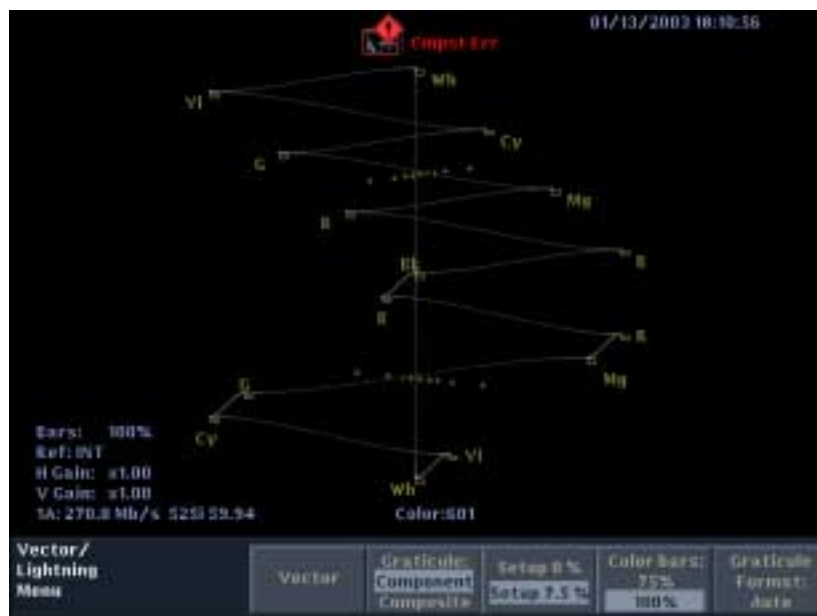
Figure 3-8: Lightning display showing proper interchannel timing
