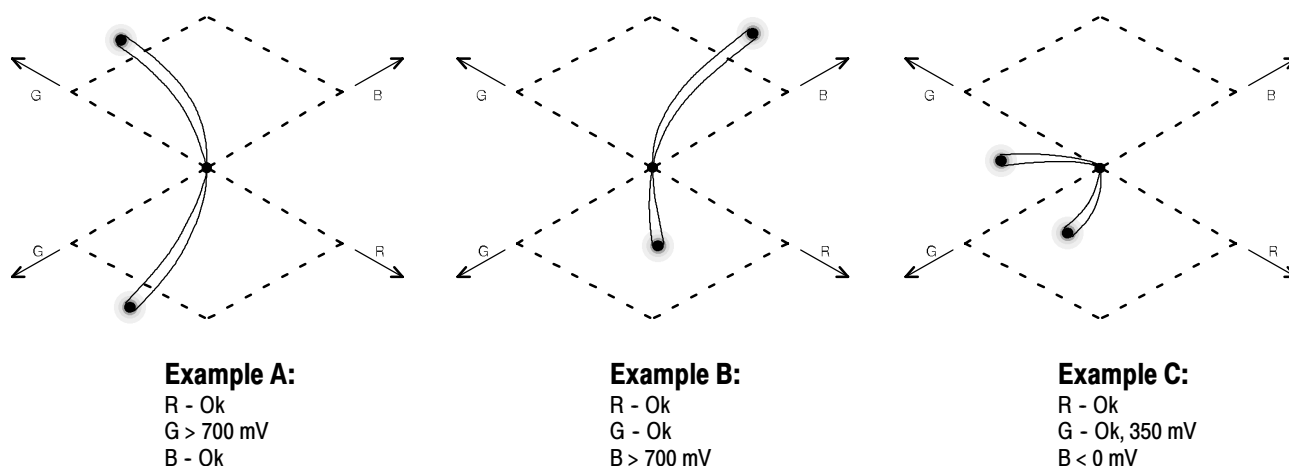
Figure 3-5: Out-of-gamut signals on a Diamond display
