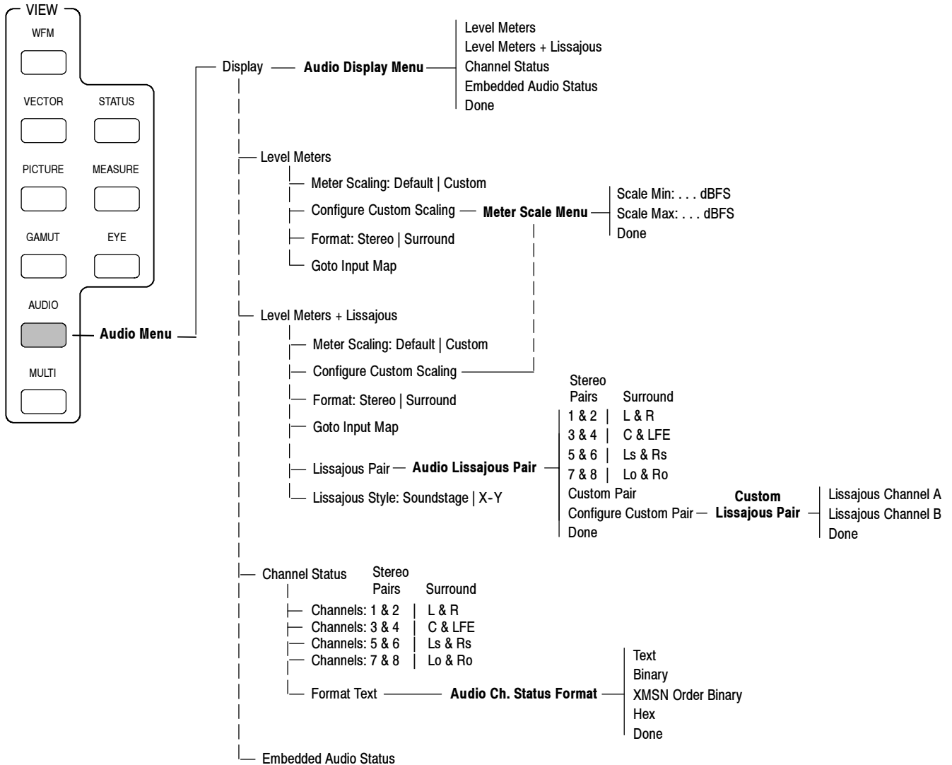
Figure 2-4: Audio menu diagram (Option DG only)
