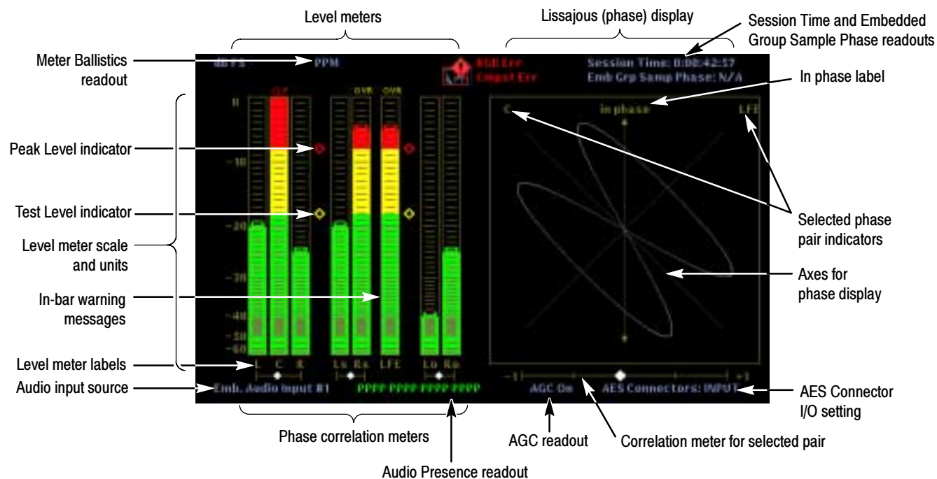
Figure 3- 1: Audio Level Meters + Lissajous display
