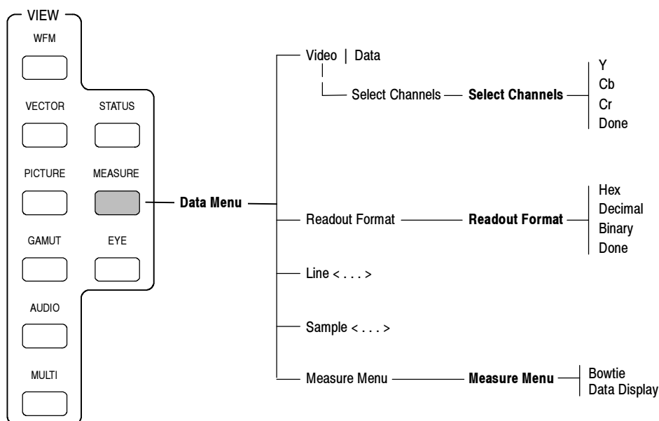
Figure 2-18: Data menu diagram
