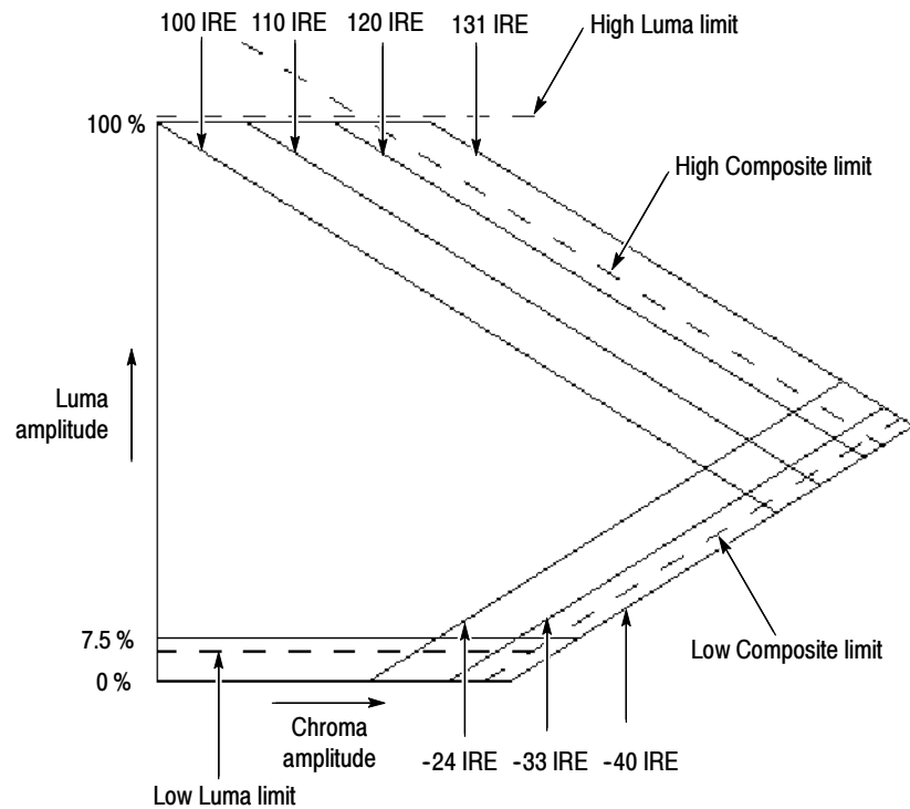
Figure 3-6: NTSC Arrowhead graticule
