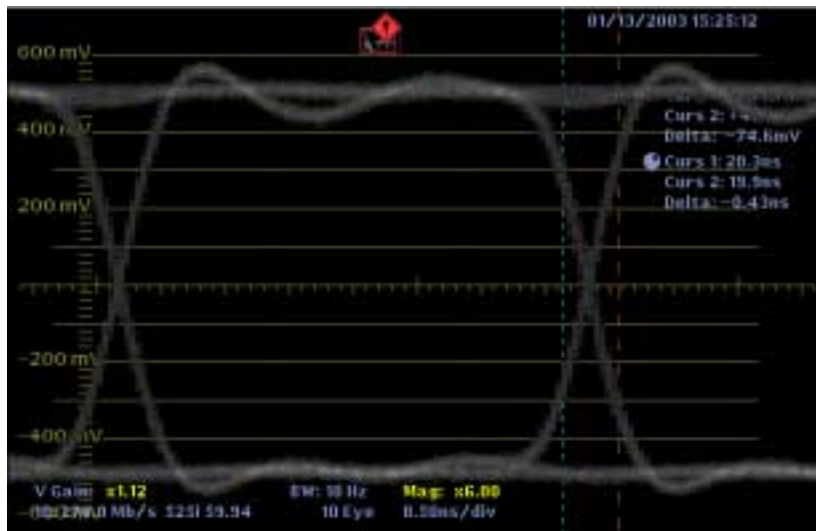
Figure 3-3: Timing Cursors alignment for measuring 20-80% rise time
