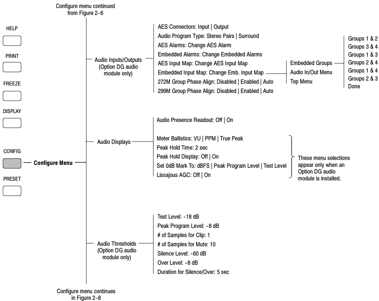
Figure 2-7: Configuration menu diagram - part 3
