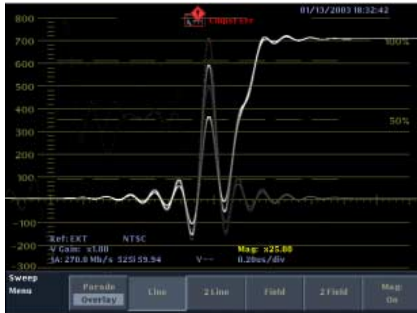
Figure 3- 10: XYZ pulse of Y channel with pass through selected
