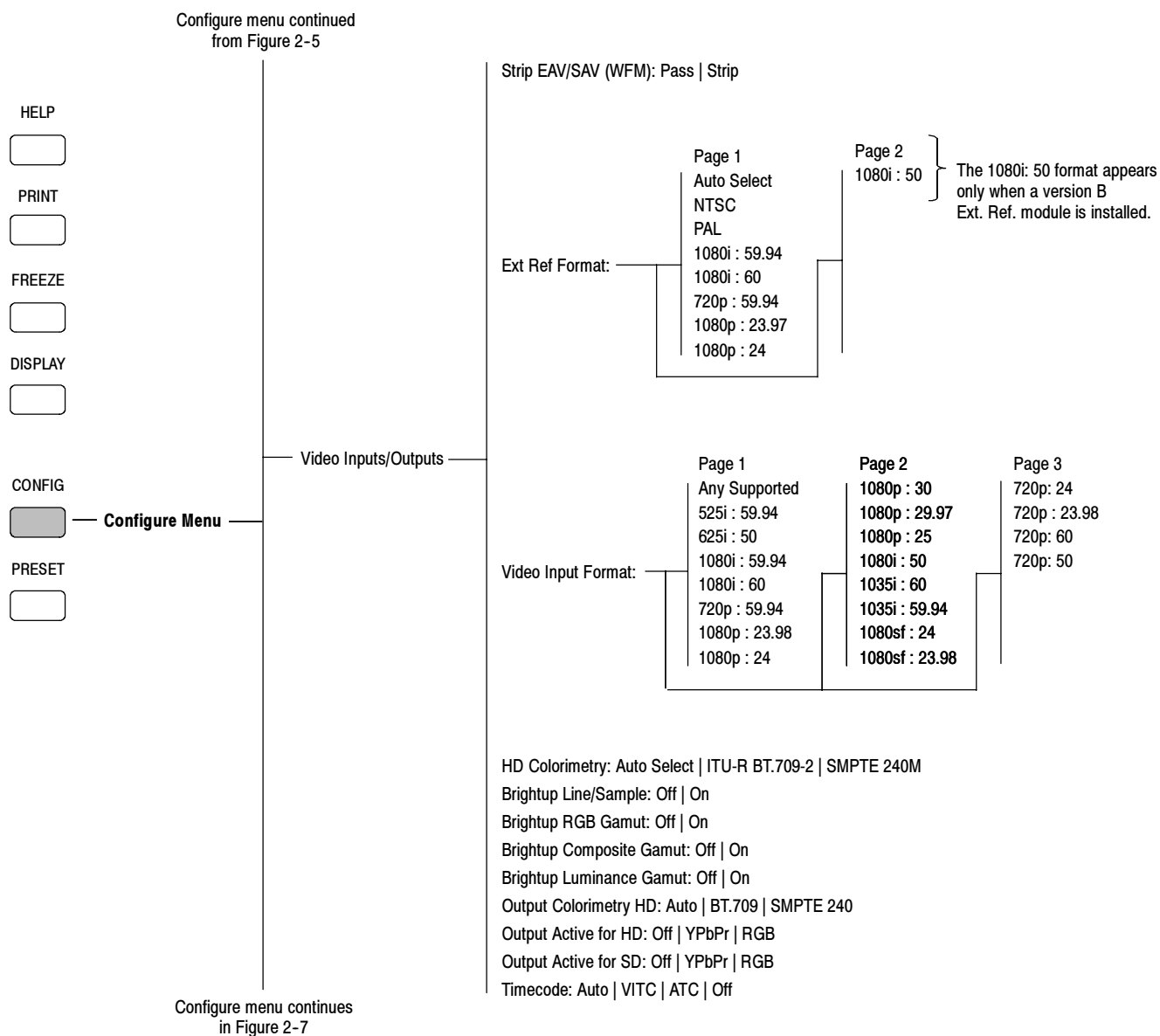
Figure 2-6: Configuration menu diagram - part 2
