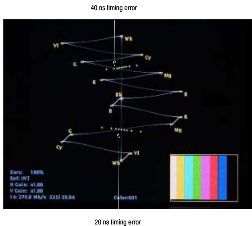
Figure 3-9: Lightning display showing interchannel timing errors
