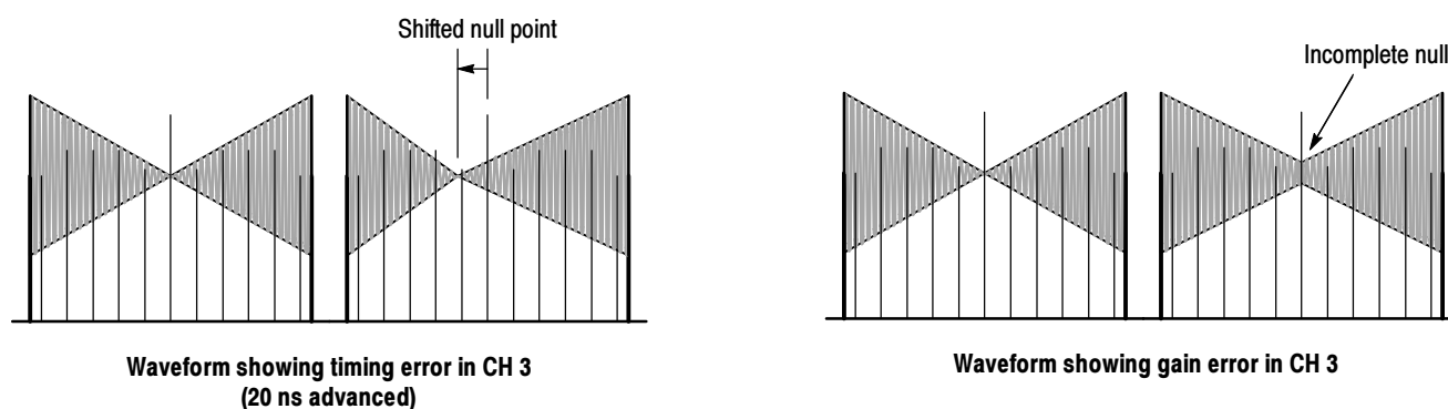
Figure 3-2: Bowtie waveforms showing timing and relative gain errors
