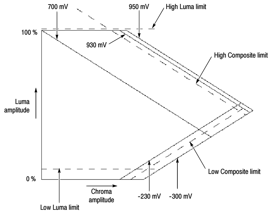
Figure 3-7: PAL Arrowhead graticule
